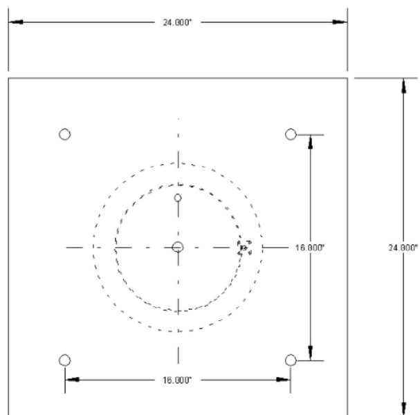
Mounting Dimensions
